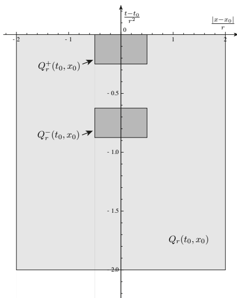
FIGURE 2. The intrinsic cylinders Q_r(t_0, x_0) , Q_r^+(t_0, x_0) and Q_r^-(t_0, x_0) .
